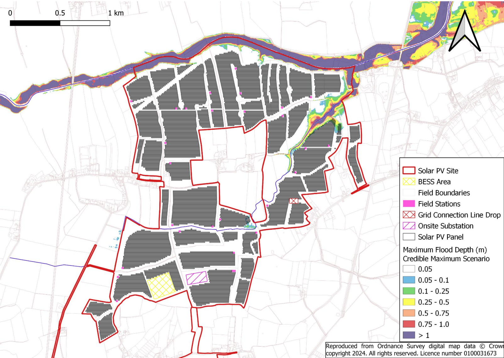
Plate 5-2: Maximum flood depth for the 1% AEP + 38% climate change event
