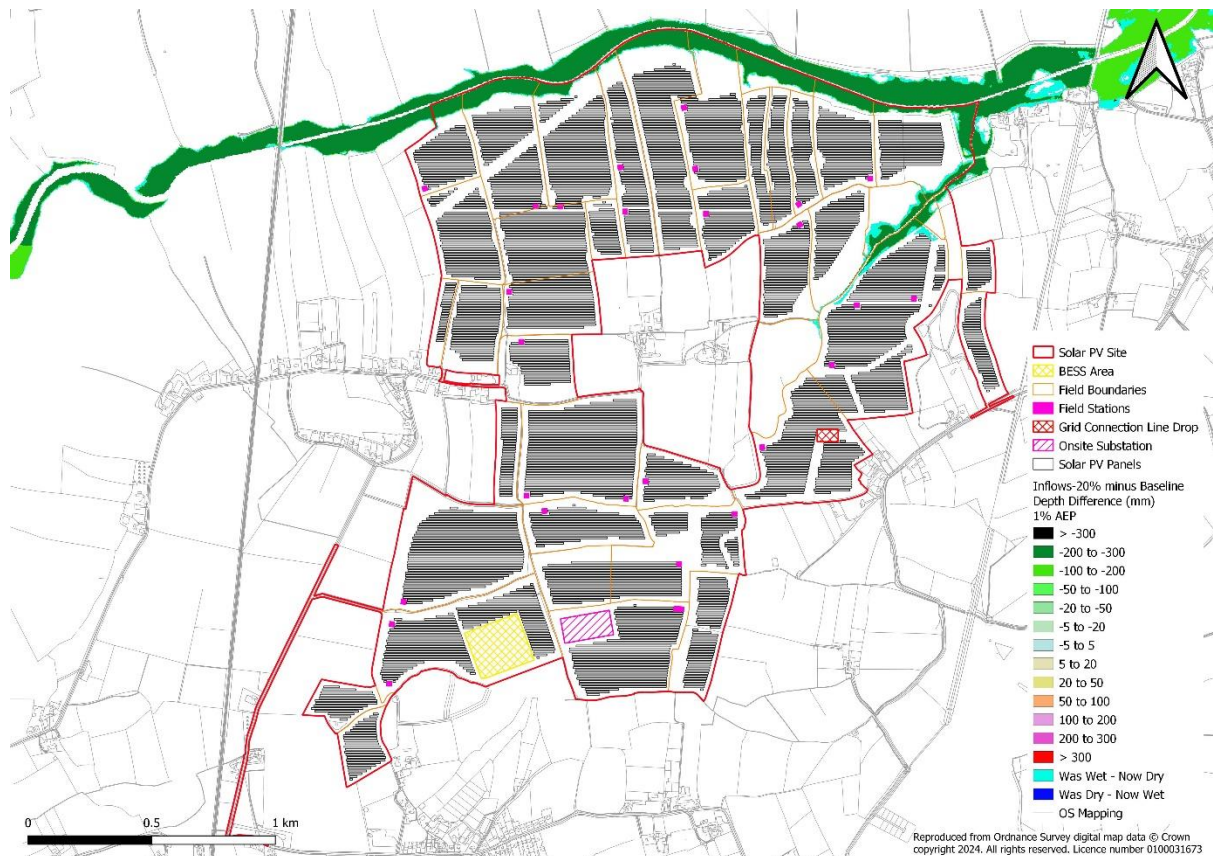
Plate 6-4: Maximum Depth Difference, Model Inflow -20% vs. Baseline (1% AEP)
