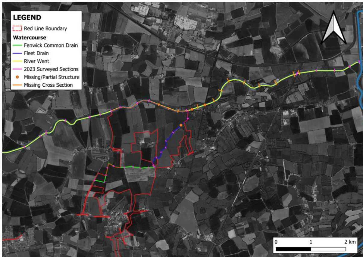
Plate 2-2: Surveyed cross-sections and structures
