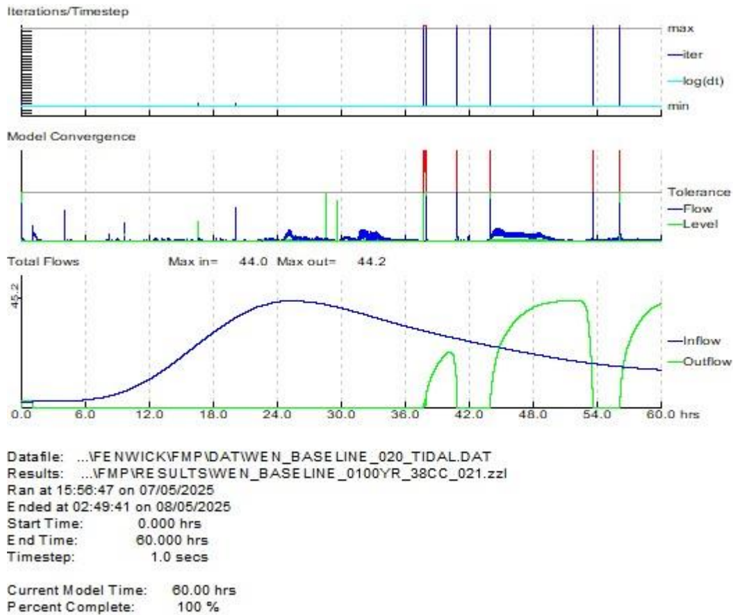
Plate 4-2: 1% AEP plus 38% climate change convergence plot
