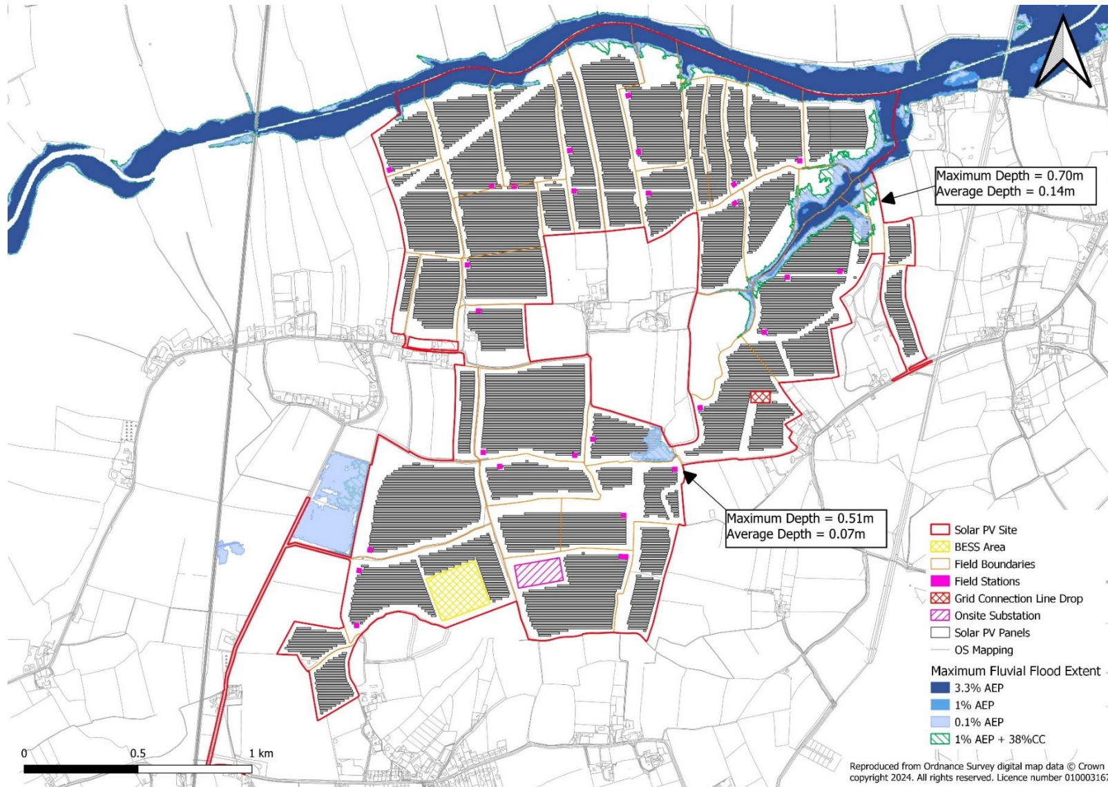
Plate 5-1: Maximum flood extents for the 3.3% AEP, 1% AEP + 38% climate change and 0.1% AEP events
