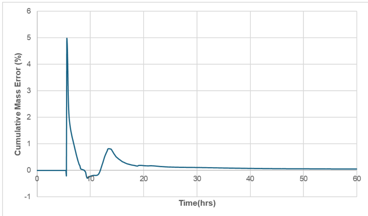
Plate 4-3: 2D Mass Balance Error for 1% AEP + 38% climate change
