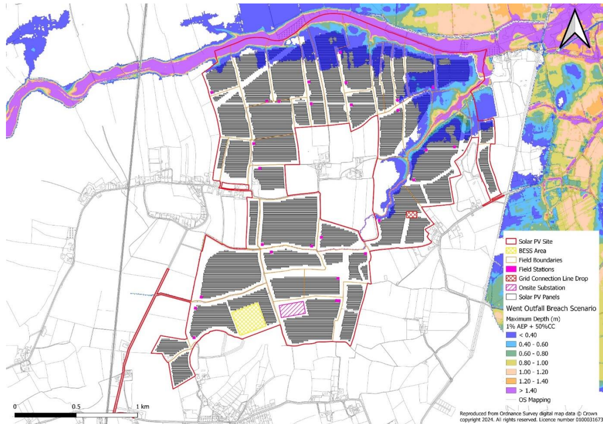
Figure 8-2: Went Outfall Breach Flood Depth 1% AEP + 50%CC
