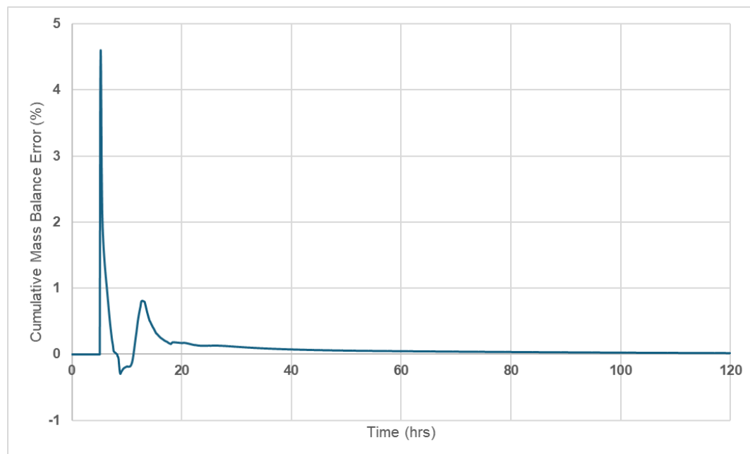
Plate 6-7: 2D Mass Balance Error for Credible Maximum Scenario
