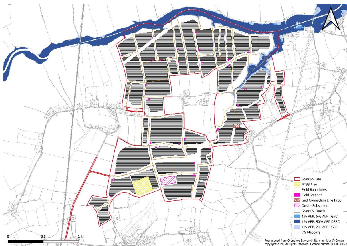
Plate 6-5: Downstream Boundary Sensitivity Test Extent Comparison
