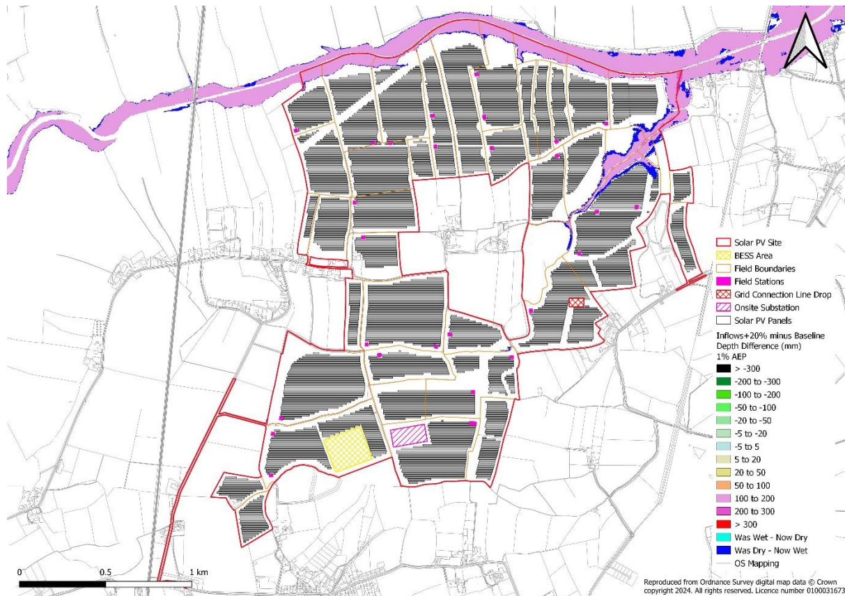
Plate 6-3: Maximum Depth Difference, Model Inflow +20% vs. Baseline (1% AEP)
